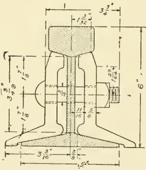
Fig. 223. Shanghai T Rail
